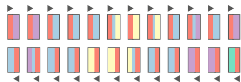
Paired-end reads
