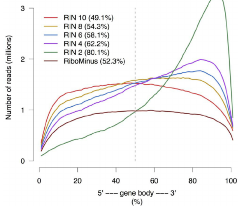
Gene body coverage
