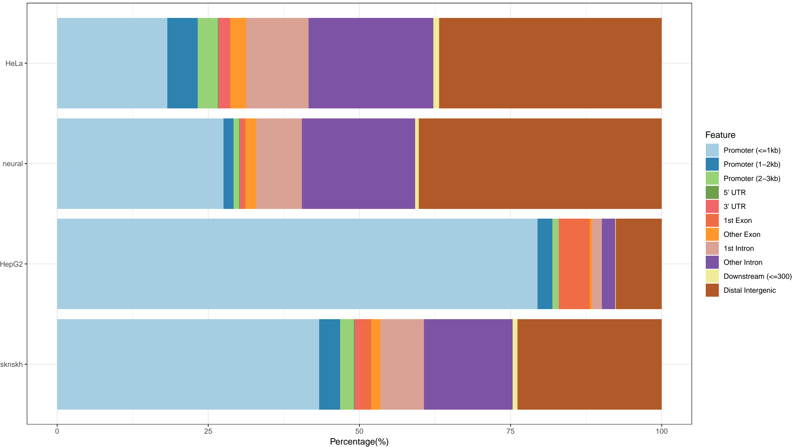
Feature Distribution
